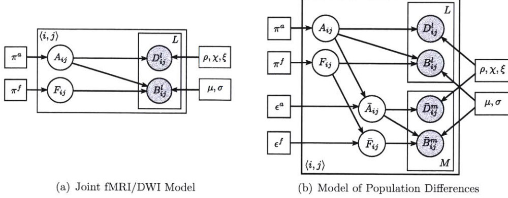
Figure 3-1: (a) Joint connectivity model for a single population. A_{ij} represents the latent anatomical connectivity between regions i and j , and F_{ij} denotes the corresponding latent functional connectivity. D_{ij}^l and B_{ij}^l are the observed DWI and fMRI measurements, respectively, between regions i and j in the l^{\text{th}} subject. (b) Joint model for the effects of schizophrenia. The control population is generated according to the model in (a). The schizophrenia templates are identified by an overbar.
