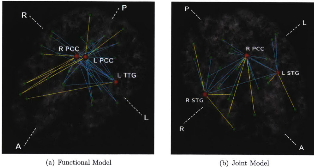
Figure 4-7: Estimated graph of functional connectivity differences. The red nodes indicate the disease foci. Blue lines indicate reduced functional connectivity and yellow lines indicate increased functional connectivity in the schizophrenia population.
