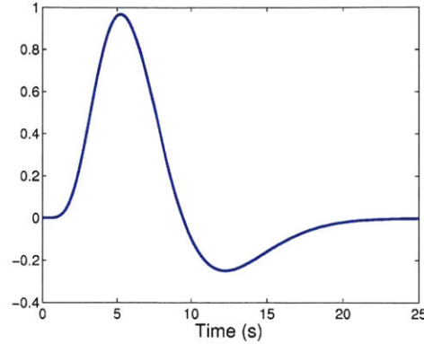
Figure 2-1: Parametric form of the Hemodynamic Response Function.
