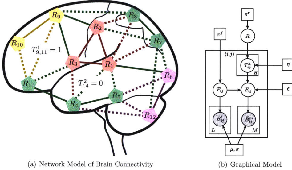
Figure 5-1: (a) Latent organization of the disorder. The nodes correspond to regions in the brain, and the lines denote pairwise functional connections. Only a subset of edges is shown; the model is defined on the full graph of pairwise connections. The green nodes and edges correspond to the healthy regions and connections, respectively. The red, yellow and purple nodes represent three clusters of disease foci, and the colored edges specify pathways of abnormal functional connectivity. The solid lines are deterministic given the region labels; the dashed lines are probabilistic. (b) The corresponding graphical model. R specifies disease cluster labels. F_{ij} denotes the latent functional connectivity between regions i and j . B_{ij}^l is the observed fMRI measurements in the l^{\text{th}} subject. Variables associated with the clinical population are identified by an overbar.
